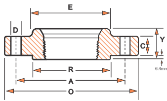
THREADED
