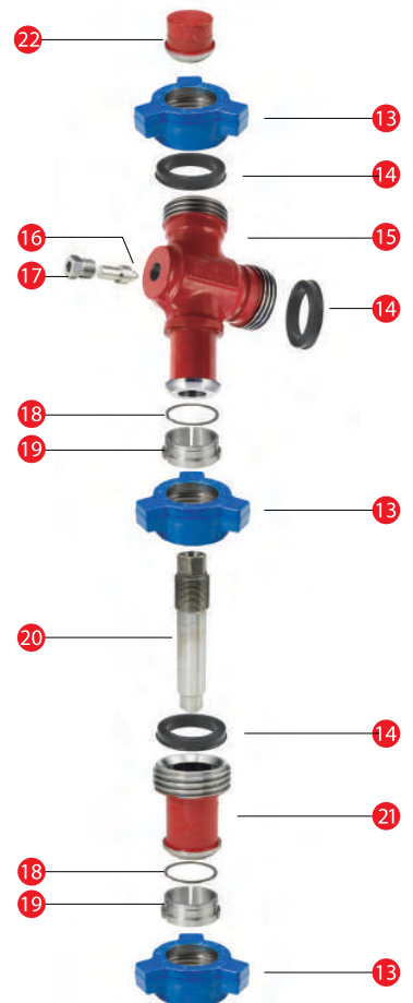
3" 1502 Adjustable Choke Valve
