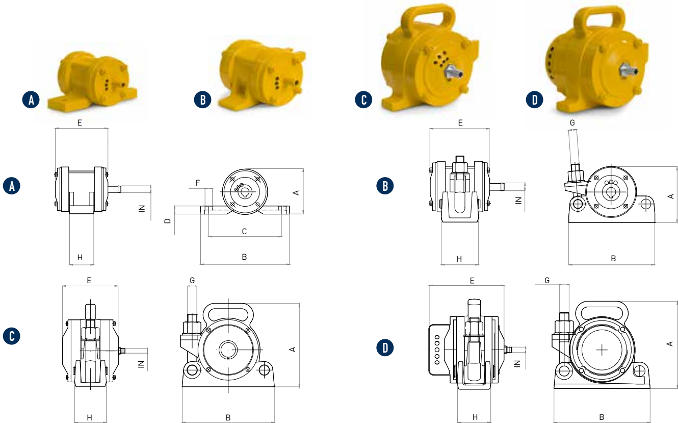
OVERALL DIMENSIONS
