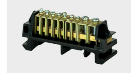
Connector 7x2 mm Product Code:- FCCN-07 Material :- Housing Polyamide. Terminal Bar Brass. Connector M.S. List Price: 221.00
