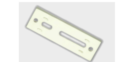
Terminal Base Product Code FCNLBN-04 -LW(80x15mm) FCNLBN-05 -LW(25 x 15mm) Suitable for 15 mm Width Open Length Terminal Material :- Polyamide List Price: 9.50
