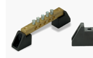
Terminal Base - Height-19mm Product Code FCNLBD-02-DMC FCNLBP-02-Polyamide FCNLBB-02-Bakelite Material :- DMC/Backalite/Polyamide. List Price:9.50
