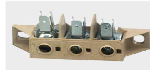
Mains Power Connector. 40Amps. 450V Product Code:- FCMPC-01 List Price: 192.00
