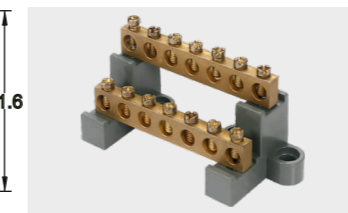
Terminal Base Product Code: FCNLB-07 - STEP Material: Polyamide Inserts- Brass-M5 List Price: 100.00
