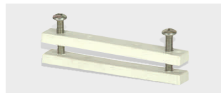
Current Transformer Cable Clamp Product Code FCCTH-01 List price: 29.50 FCCTH-02 List price: 35.50 Size:- 82 /115 mm Material :- Polyamide.
