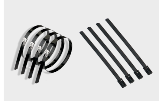
STAINLESS STEEL CABLE TIES (UN COATED) Ball - Self Locking Operating Temperature : - 80°C to 538°C Tensile Strength : 105 Kg.
