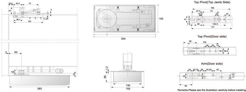
Assembling picture of floor hinge series
