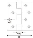
M.S.Hinges ( GP finish ) 4x3x3.0 & 5x3x3.0 Finish: Gold Materials: Iron
