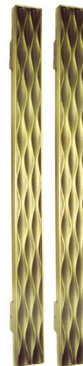
DH-935 Material: Aluminum color: AB Size: 35x32x420mm
