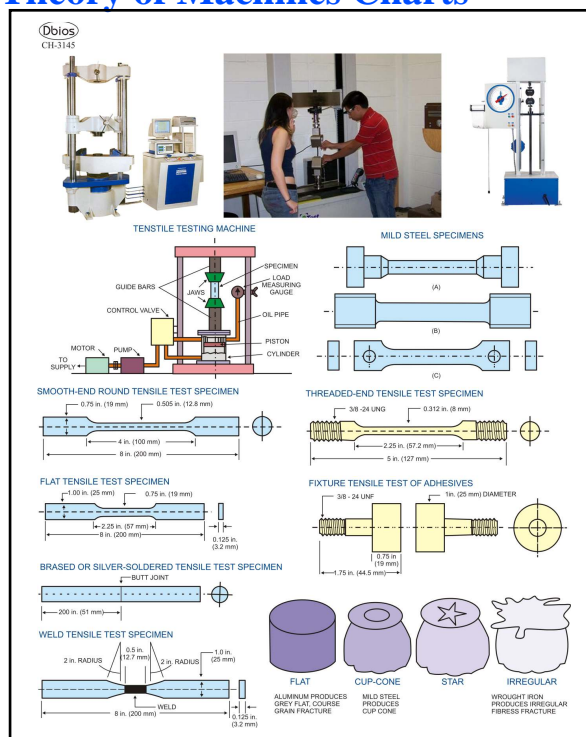
CH 3145 DRAWING OF UTM (MACHINE & SAMPLES)
