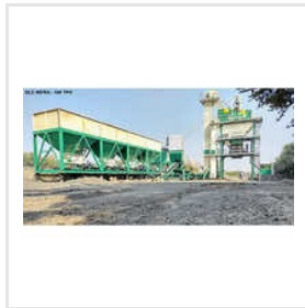
160 Tph Industrial Asphalt Batch Mix
