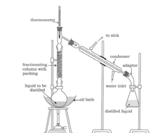
Fig.12.6 Fractional distillation. The vapours of lower boiling fraction reach the top of the column, first followed by vapours of higher boiling fractions.
