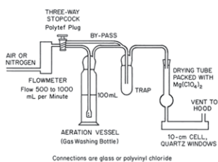
Mercury Aeration Apparatus
