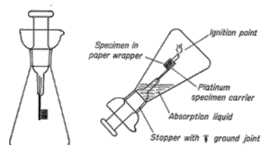
Oxygen Combustion Flask
