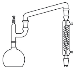
Fluoride Distillation Apparatus
