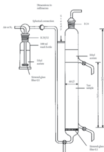
Gas Stripping Apparatus Column / Sublation Apparatus
