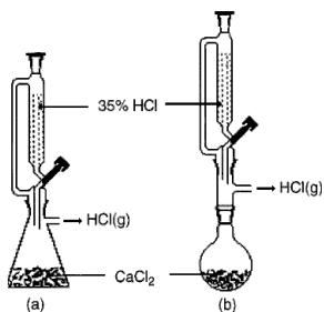
Dry HCL Generation Unit
