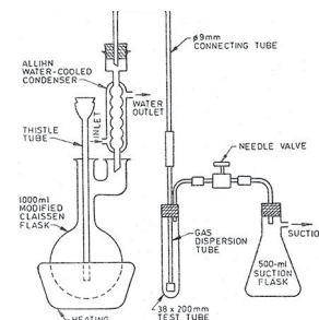
Cynide Distillation as per I.S. 3025
