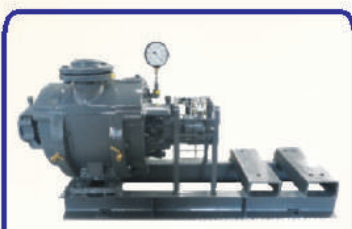
Single Stage Vacuum Pump Maximum Capacity : 1500 M 3 /hr. Maximum Vacuum : 710 mm to Hg
