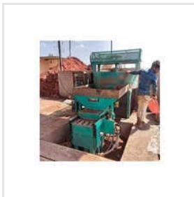
Semi Automatic Fly Ash Brick Machine
