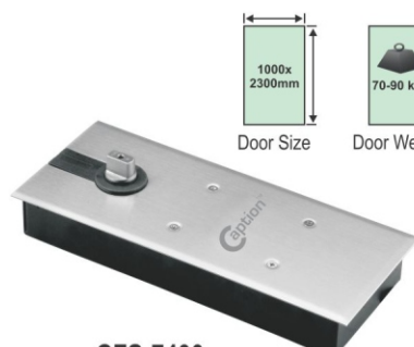
CFS-7400 Single Spring Floor Hinge
