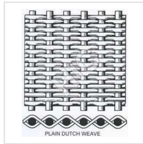
Plain Dutch Weave
