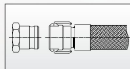
CAMLOCK COUPLING TYPE HF10
