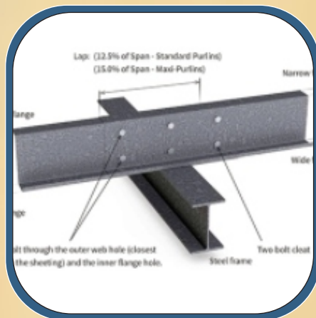
Purlins
