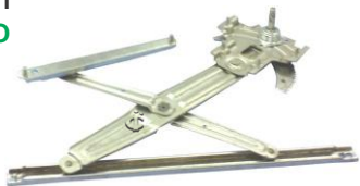
WINDOW REGULATOR MANUAL FRONT
