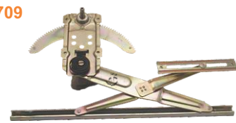
WINDOW REGULATOR L/R LPT 709
