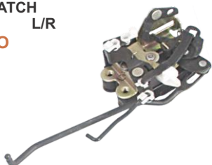
DOOR LOCK ASSY. FRONT ACCENT
