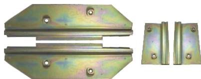
GLASS CHANNEL FRONT/REAR INDICA
