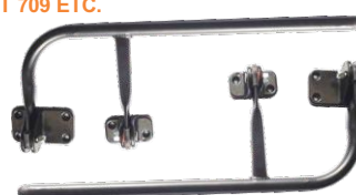
SIDE MIRROR ROD WITH BRACKET R/L LPT 709 ETC.
