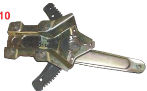
POWER WINDOW REGULATOR FRONT RITZ
