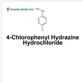
4-Chlorophenyl Hydrazine
