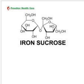
Iron Sucrose
