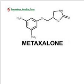
METAXALONE
