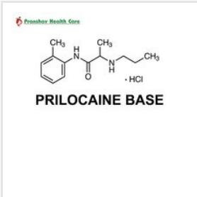
PRILOCAINE BASE
