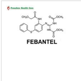
Febantel
