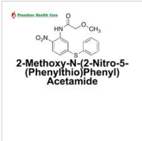
2-Methoxy-N-(2-Nitro-5-Nitro-5-
