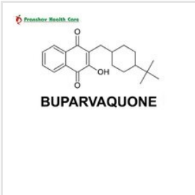
BUPARVAQUONE Ingredients
