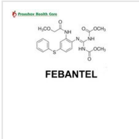
Febantel USP
