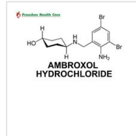
Ambroxol Hydrochloride
