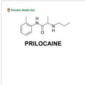
Prilocaine
