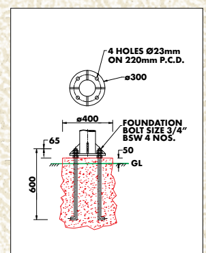
Installation Schematics
