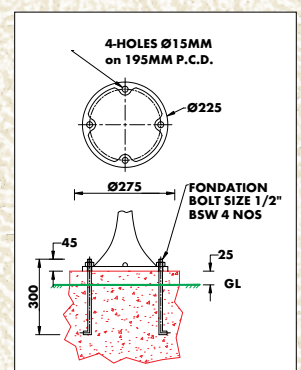
Installation Schematics
