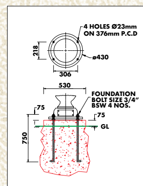
Installation Schematics
