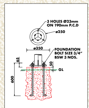
Installation Schematics
