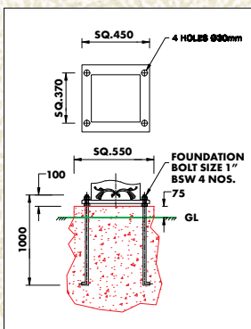
Installation Schematics
