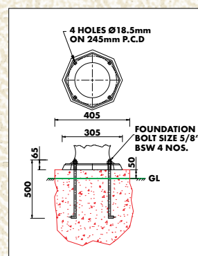
Installation Schematics
