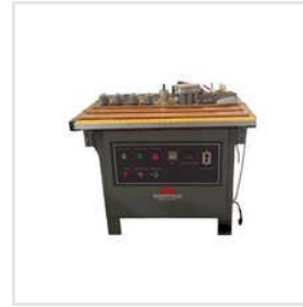
Economic Manual Edge Bander Machine
