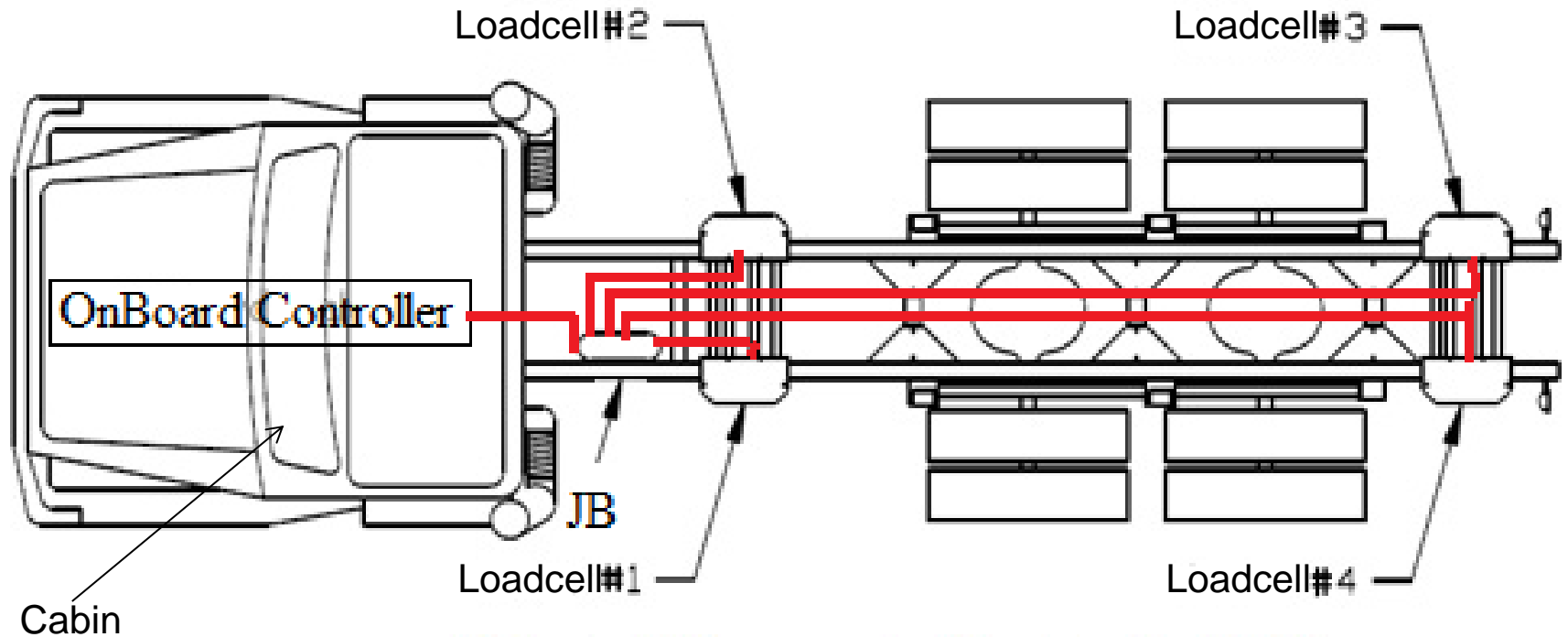
Four point loadcell connections
