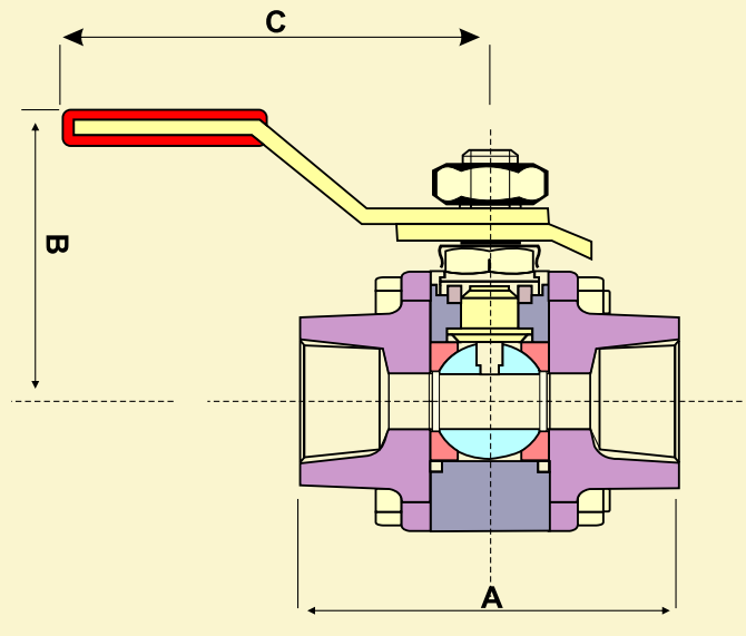
SCREWED END
