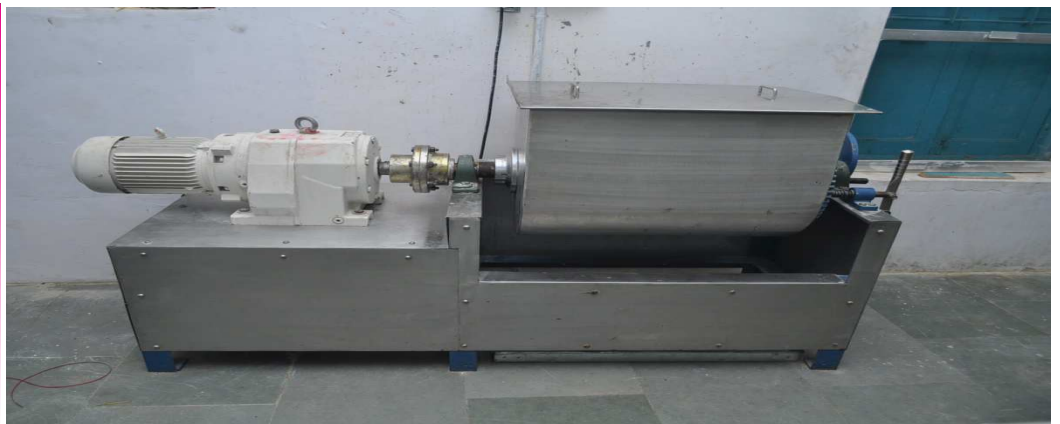
(1). FLOUR KNEADING MACHINE (Two In One) (2). FLOUR KNEADING MACHINE (Heavy Duty In Line).
