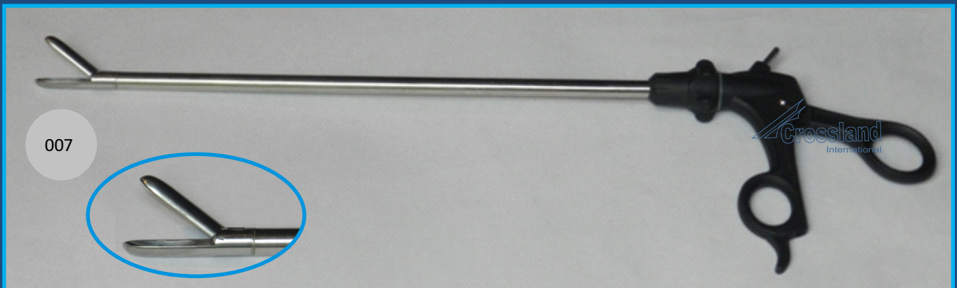
(001) : CL-LAP-001 : Universal Grasper Forceps. 5 mm. Rotatable & detachable.
