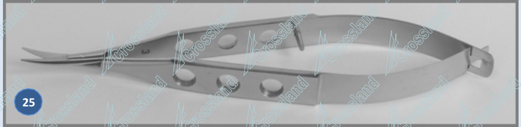
CASTROVIEJO CORNEAL SCISSORS: GENTLY CURVED : OVERALL LENGTH 113 mm. SMOOTH TIP FROM MID SCREW TO TIP 13 mm BLADE. FLAT THREE HOLE BODY. (CL-SC-02)
