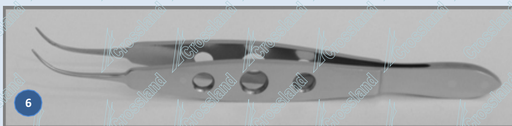
CASTROVIEJO TYING FORCEPS. CURVED: OVERALL LENGTH 115 mm. THREE HOLE BODY. TYING PLATFORM 6 mm / 10 mm. DULL FINISH. SMOOTH CURVED. (CL-FR-05)
