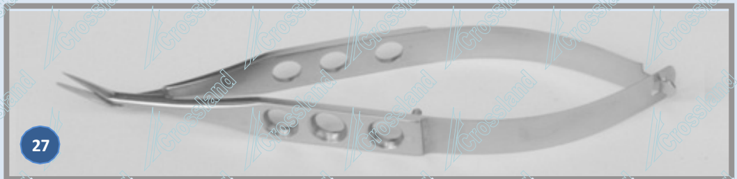
CASTROVIEJO CORNEAL SCISSORS. ANGLED : OVERALL LENGTH 113 mm SHARP TIP. 11 mm LONG ANGLED BLADES. FLAT THREE HOLE BODY. (CL-SC-02 /AN).
