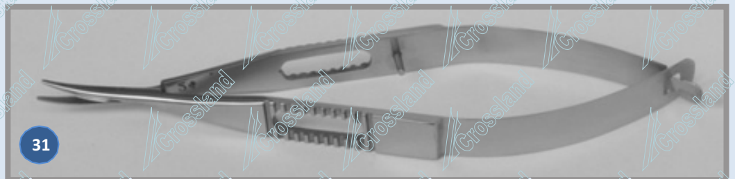
WESTCOTT SCISSORS. Perforated handle : OVERALL LENGTH 110 mm. BLUNT TIP. FROM MID SCREW TO TIP 14 mm CURVED BLADE. (CL-SC-05 /P)
