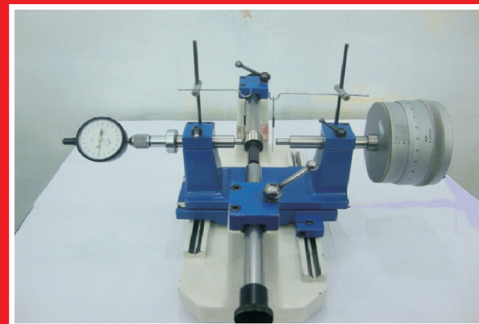
Floating Carriage Diameter Measuring Machine (FCDM).
