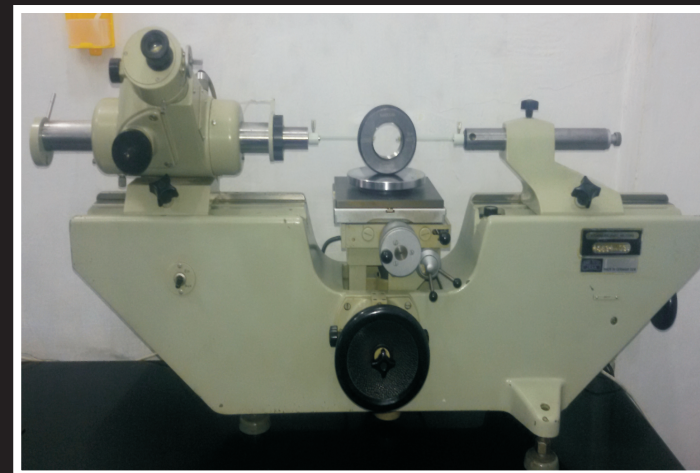
Carl Zeiss - Length Measuring Machine for internal & external measurement - Range upto 300mm.
