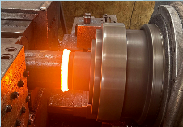
• FRICTION WELDING
