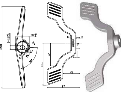
Aluminum alloy twin pedal with hexagonal hole
