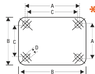
Wheel Structure
