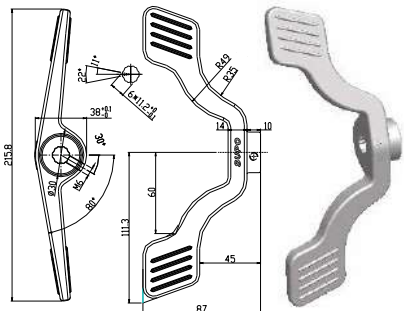
Aluminum alloy twin pedal with quincuncial hole
