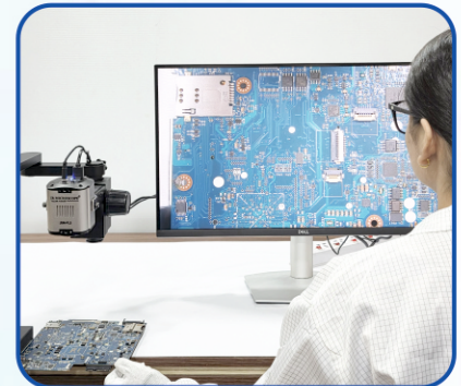
4k Digital Autofocus Camera JBM-PL5
