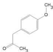
P-Methoxyphenyl Acetone
