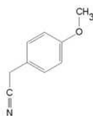
P-Methoxyphenyl Acetonitrile
