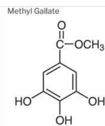
Methyl Gallate
