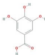
Gallic Acid
