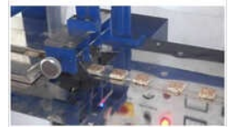
Chikki Packing Machine
