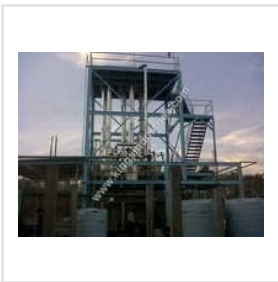
MEE Wastewater Evaporators
