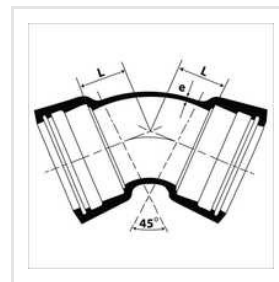
45 Degree Double Socket Bend
