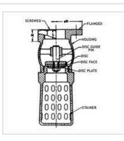
Cast Iron Foot Valve
