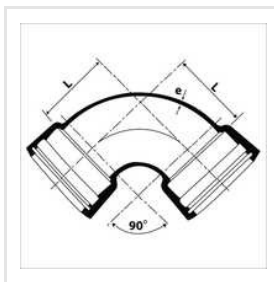
90 Degree Double Socket Bend
