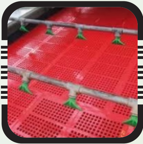
Polyurethane Screen Panel
