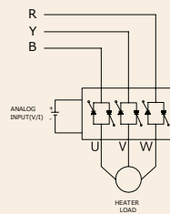
Schematic
