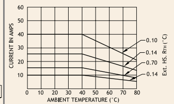
Derating Curve
