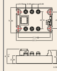
Mechanical Drawing
