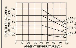
Derating Curve
