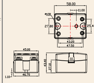
Mechanical Drawing
