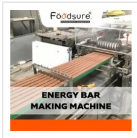
Energy Bar Making Machine
