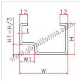
6-9 Mtr Pressed Steel Door Window Section
