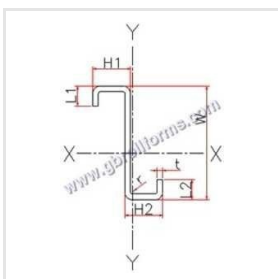
Z Purlin
