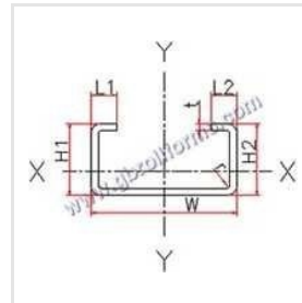
Lip Channel
