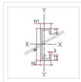
C Purlin
