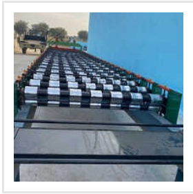
Industrial Mild Steel Roll Forming Machine
