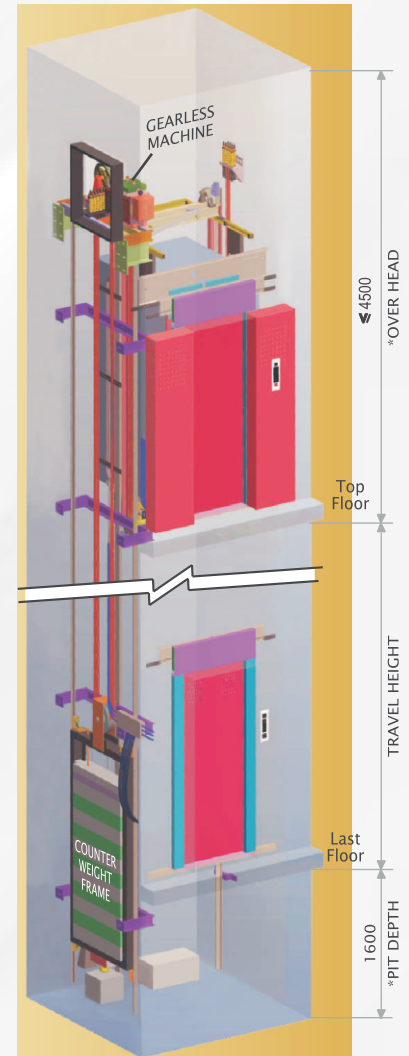
(SECTION : A-A) LIFT WELL
