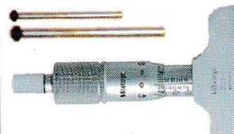
Depth Micrometer
