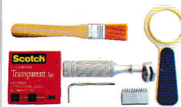
Cross Hatch Cutter (1mm / 2mm / 3mm) Adhesion Tape
