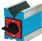
Magnetic V Block (3", 4", 6") 53
