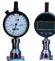
Dial & Digital S/c Profile Gauge 0.001mm
