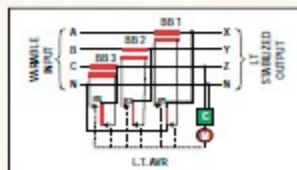
Inner View of Unbalanced Stabilizer
