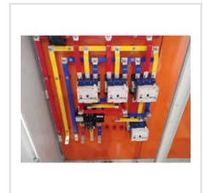
Star Delta Control Panel
