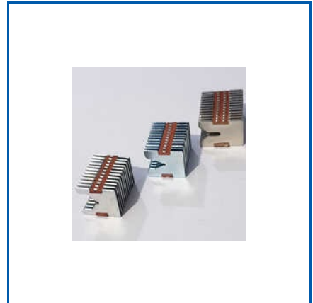
MCB ARC CHUTE ASSEMBLY
