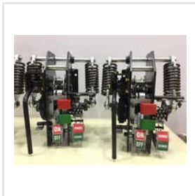
Spring Charging Mechanism
