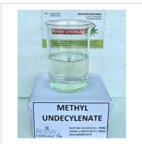
Methyl Undecylenate
