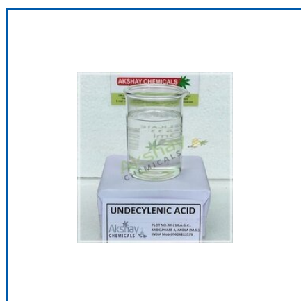
UNDECYLENIC ACID
