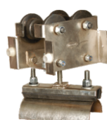
Model No. CE - 30 Four Wheel (Adjustable) Cable Clamping Dia : Multi Cable
