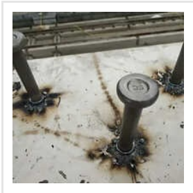
Mild Steel Shear Connector Stud
