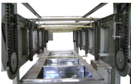
Multistage Material Handling (automatic Conveyor) Cleaning Systems Side View
