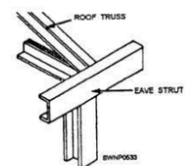
Figure 3-29.—Eave strut.
