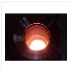
Induction Vacuum Melting Furnace
