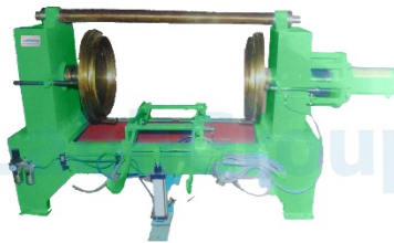
Drum Flanging Machine
